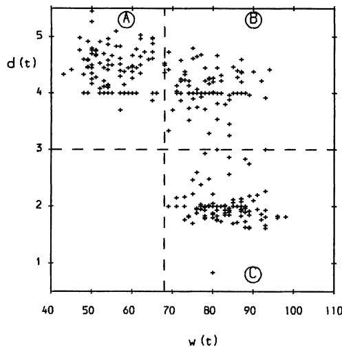
Fig. 3. Duration d_t versus previous waiting time w_t
